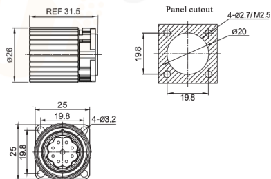
Female contact square flange receptacle
