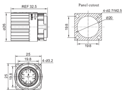
Female contact square flange receptacle
