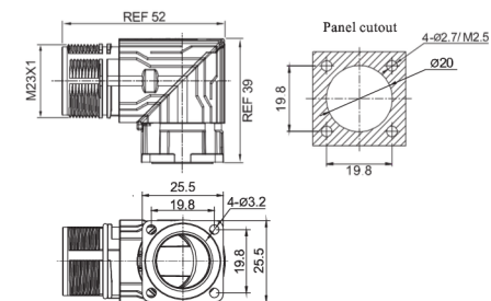
Male contact angled square flange receptacle
