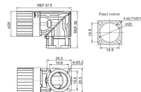
Female contact angled square flange receptacle
