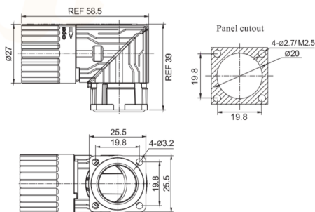
Female contact angled square flange receptacle
