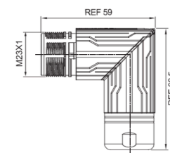
Male contact angled cable connector
