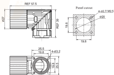
Female contact angled square flange receptacle Threaded coupling
