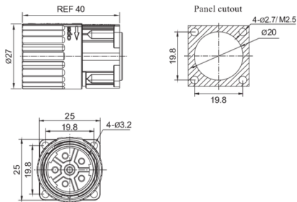
Female contact square flange receptacle Bayonet coupling
