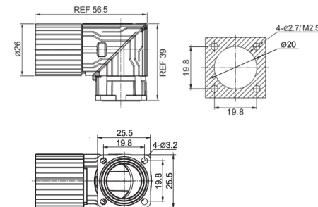
Female contact angled square flange receptacle
