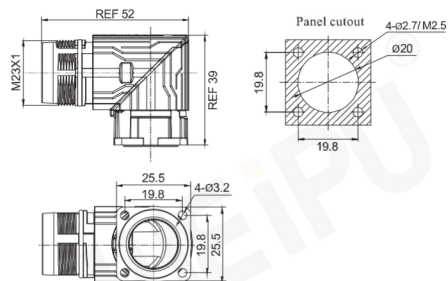
Male contact angled square flange receptacle Threaded coupling
