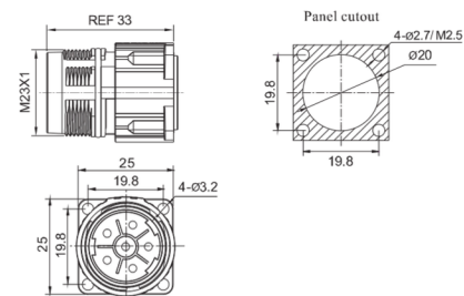
Male contact square flange receptacle Bayonet coupling
