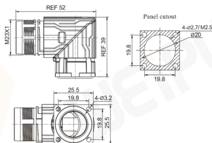
Male contact angled square flange receptacle
