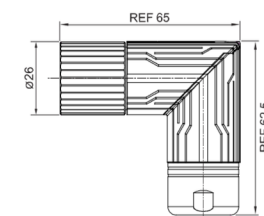
Female contact angled cable connector
