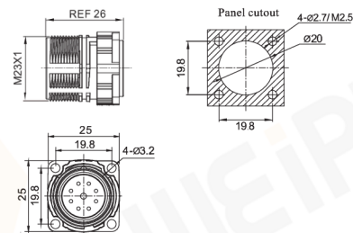
Male contact square flange receptacle
