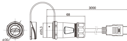
HDMI2.0 Receptacle Mate with SF2410
