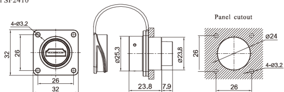
HDMI2.0 Square flange receptacle Mate with SF2410
