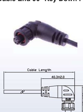
C1 Plastic Cable End 90° Key Down Female Lock Type
