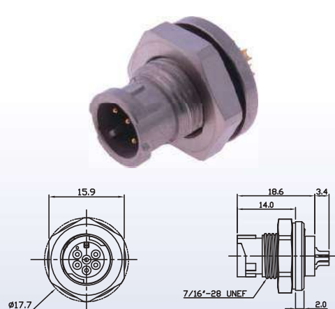
C1 Metal Panel Mount Male Lock Solder
