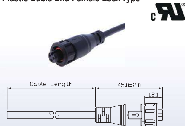
C1 Plastic Cable End Female Lock Type
